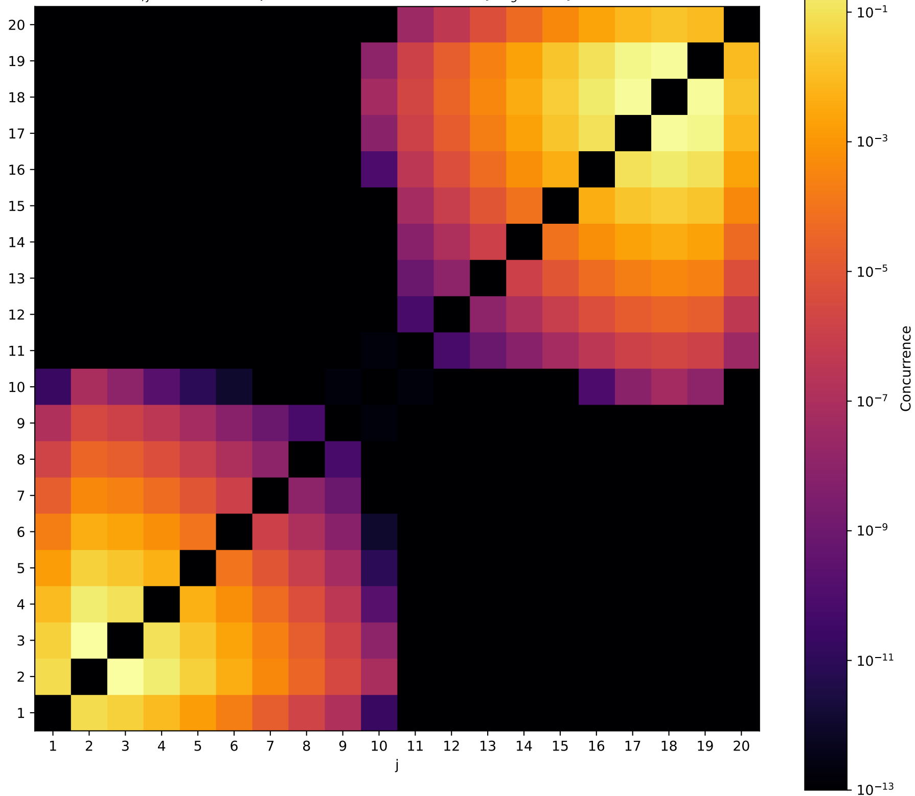
C_{i,j}(t = 0.50) for prod state (2,18) (band 2) - J_{long} = 20, J_z = 1, \alpha \rightarrow \infty
